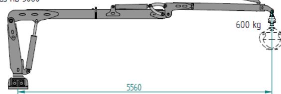
IGJ HD 5070
