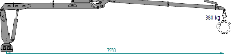
IGJ HD 5080
