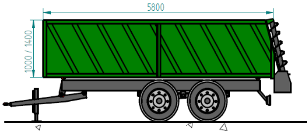
Agromax T A120 TSZ / Agromax T A140 TSZ 5,8x2,2x1,0m 5,8x2,2x1,4m
